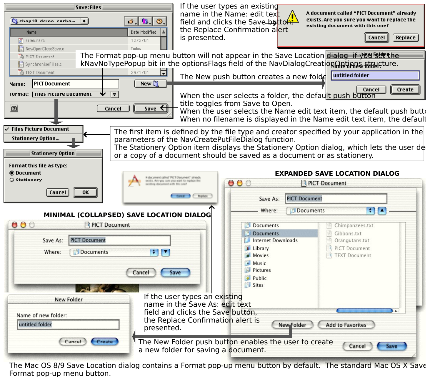
FIG 10 - THE SAVE LOCATION DIALOG BOX (PARTIAL) AND ASSOCIATED DIALOGS
