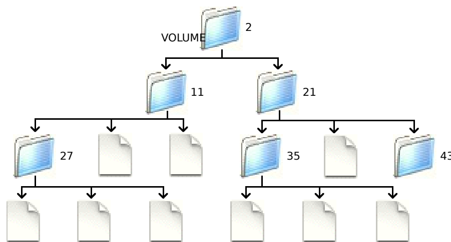
FIG 3 - MACINTOSH HIERARCHICAL FILE SYSTEM
