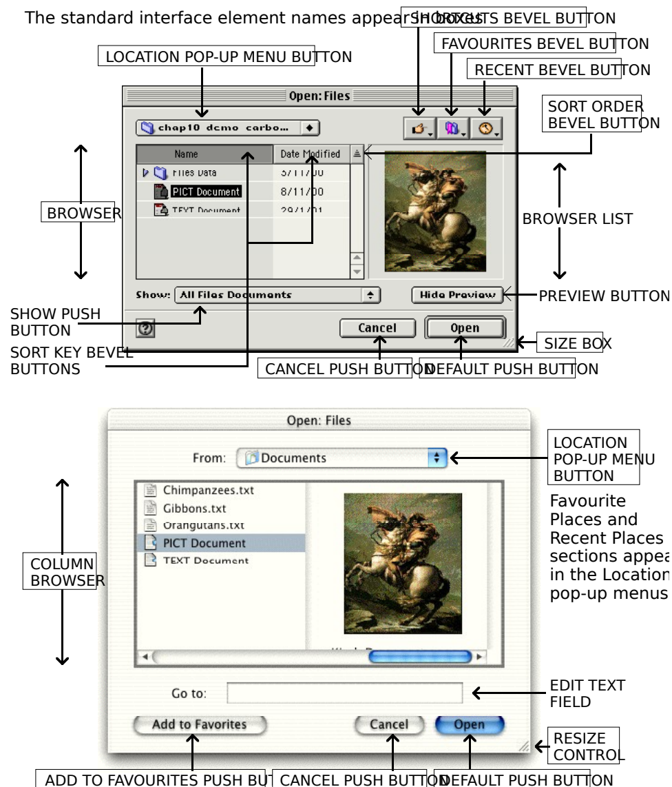
FIG 5 - STANDARD USER INTERFACE ELEMENTS IN NAVIGATION
