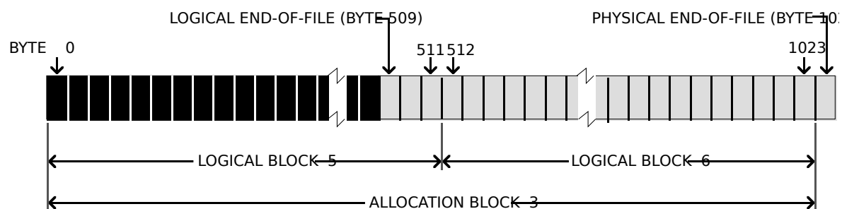
FIG 2 - LOGICAL AND PHYSICAL END-OF-FILE
