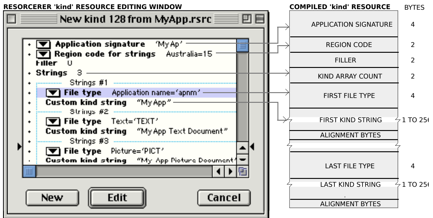
FIG 8 - STRUCTURE OF A COMPILED 'kind' RESOURCE AND CREATING A 'kind' RESOURCE
