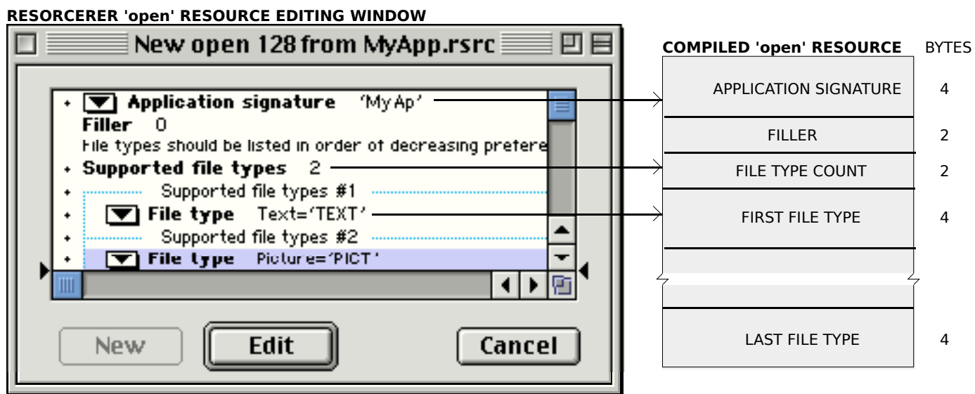
FIG 9 - STRUCTURE OF A COMPILED 'open' RESOURCE AND CREATING AN 'open' RESOU
