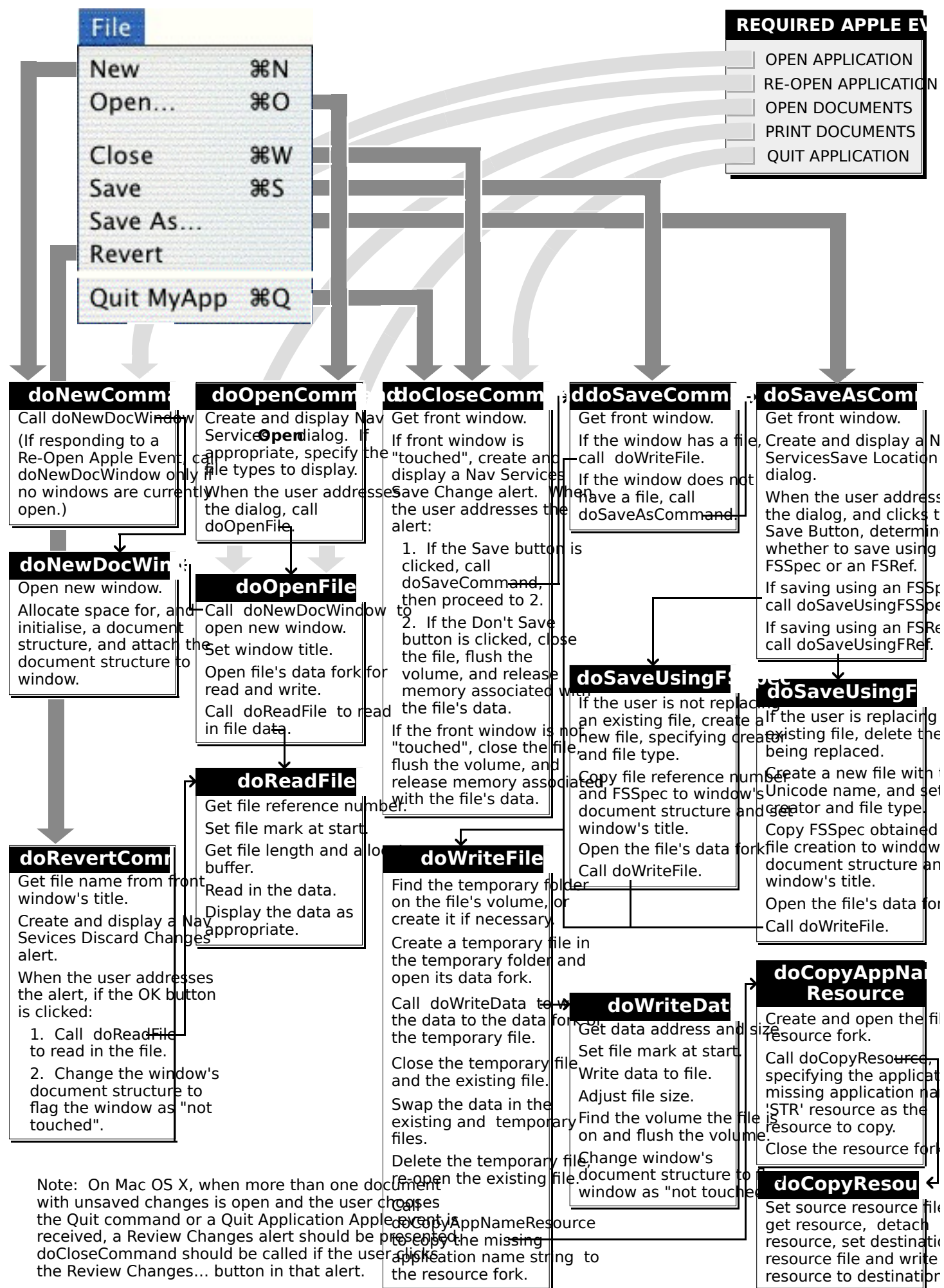
FIG 4 - GENERAL FILE MENU, QUIT ITEM, AND REQUIRED APPLE EVENTS HANDLING
